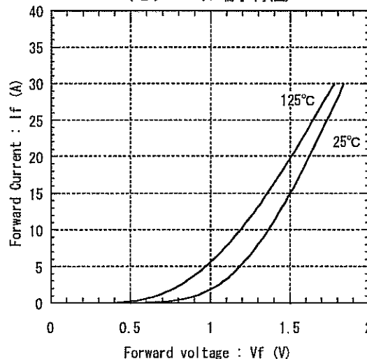
Forward current vs. Forward voltage (モジュール端子特性)
