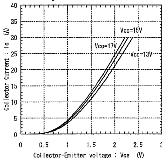
Collector current vs. Collector-Emitter voltage Tj=125°C (チップ端特性)
