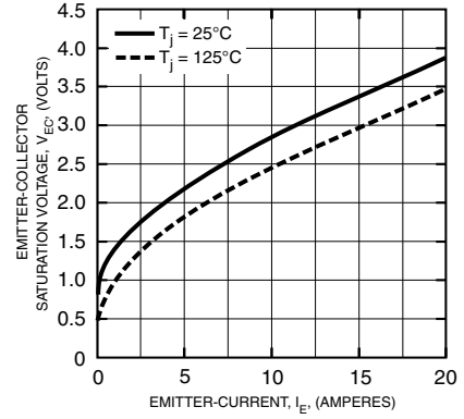
EMITTER-COLLECTOR SATURATION VOLTAGE CHARACTERISTICS (BRAKE PART - TYPICAL)
