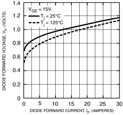
DIODE FORWARD VOLTAGE CHARACTERISTICS (CONVERTER PART - TYPICAL)
