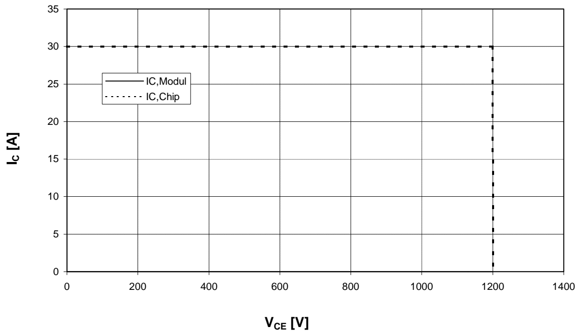
Reverse bias safe operating area Inverter (RBSOA) T_{vj} = 125^\circ\text{C} , V_{GE} = \pm 15\text{V}
