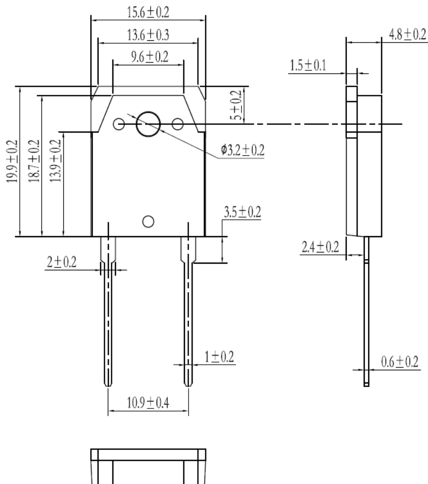
Dimensions in (mm) Figure 8. Package Outline
