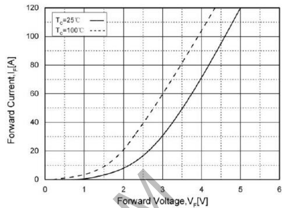
Fig. 10. Forward Characteristics
