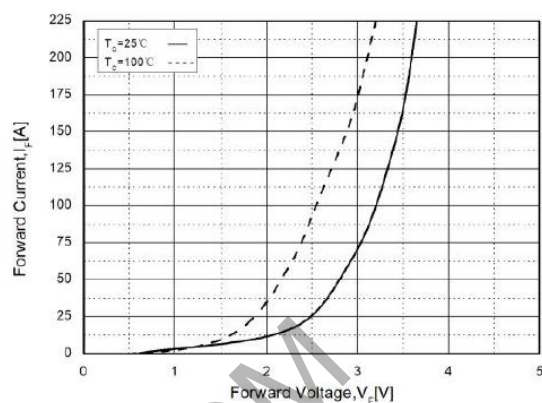
Fig. 10. Forward Characteristics
