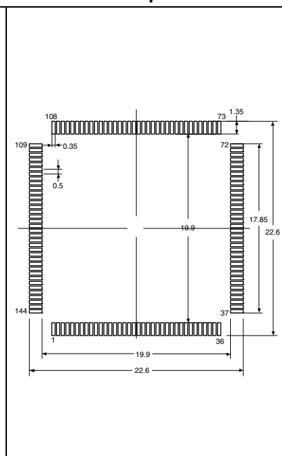
Figure 77. Recommended footprint (1)(2)
