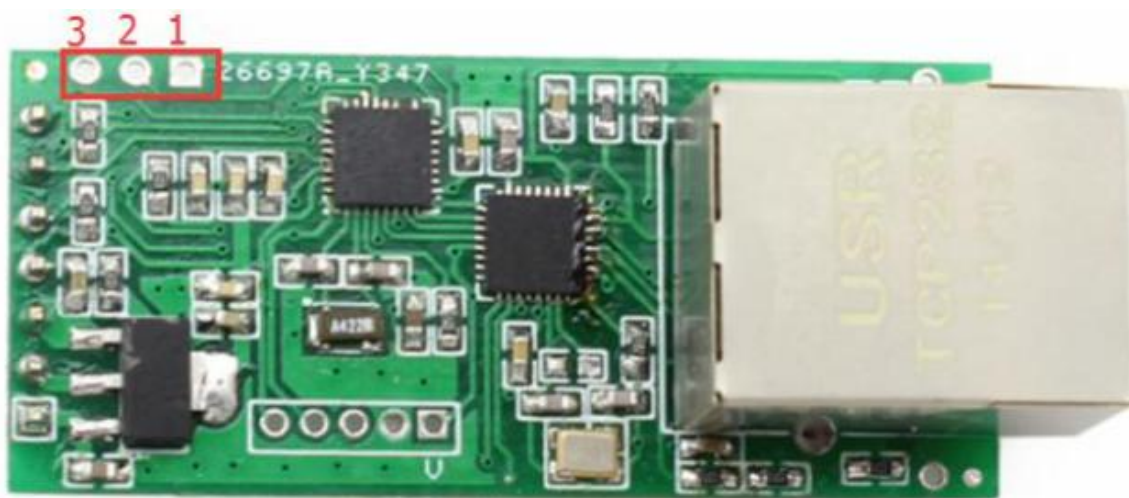
Figure 2 Pin definition
