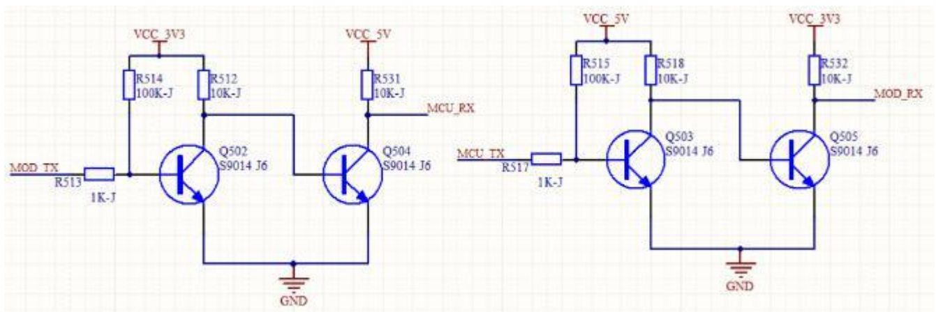
Figure 7 Switching circuit
