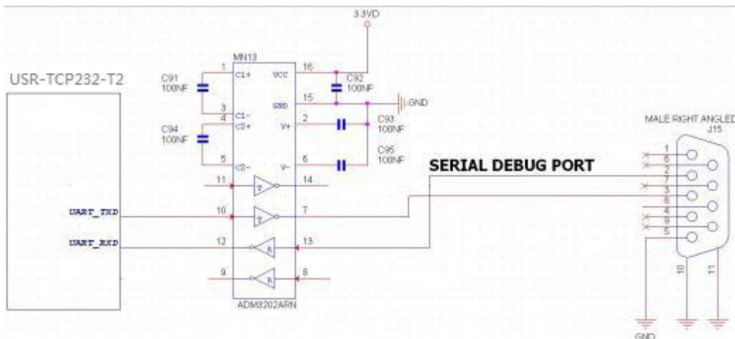
Figure 6 UART interface
