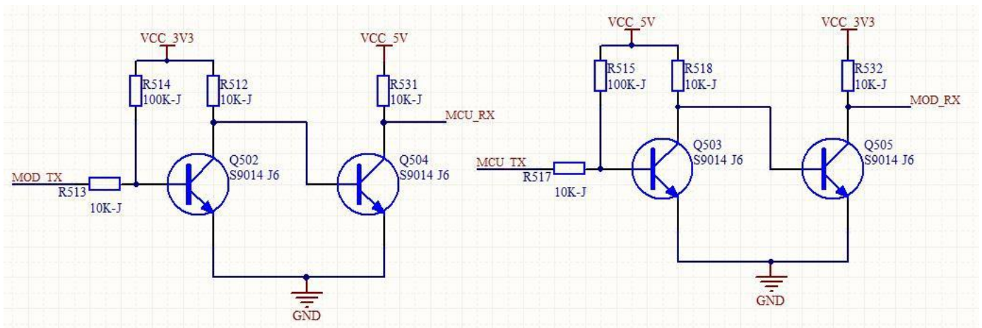
Diagram 3.1.1-2 3.3V to 5V voltage conversion circuit
