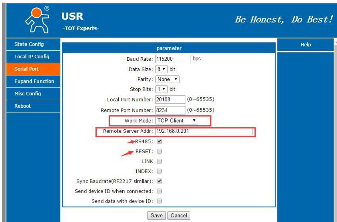
Diagram 5.2.3-1 Serial Port
