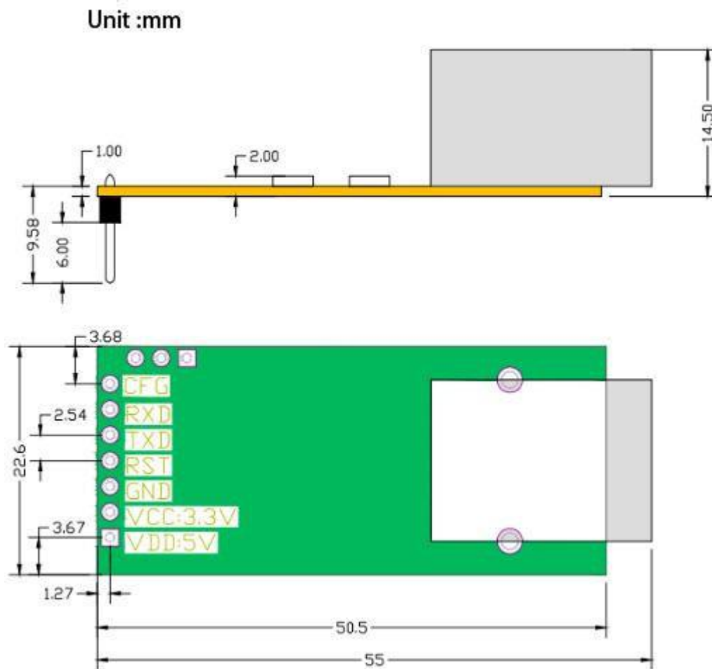
Diagram 3.1.2-1 T2 Dimension
