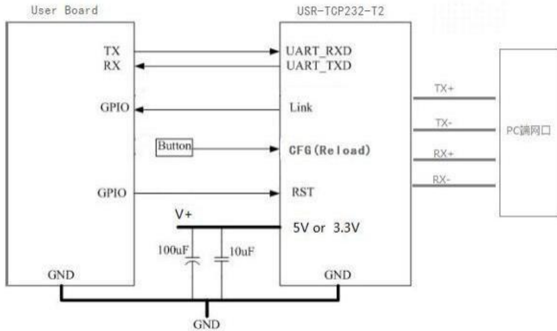
Diagram 3.2.1-1 Typical Application Connection
