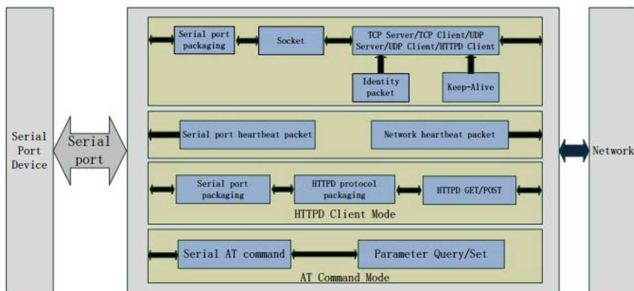
Diagram 4-1 Module Functions
