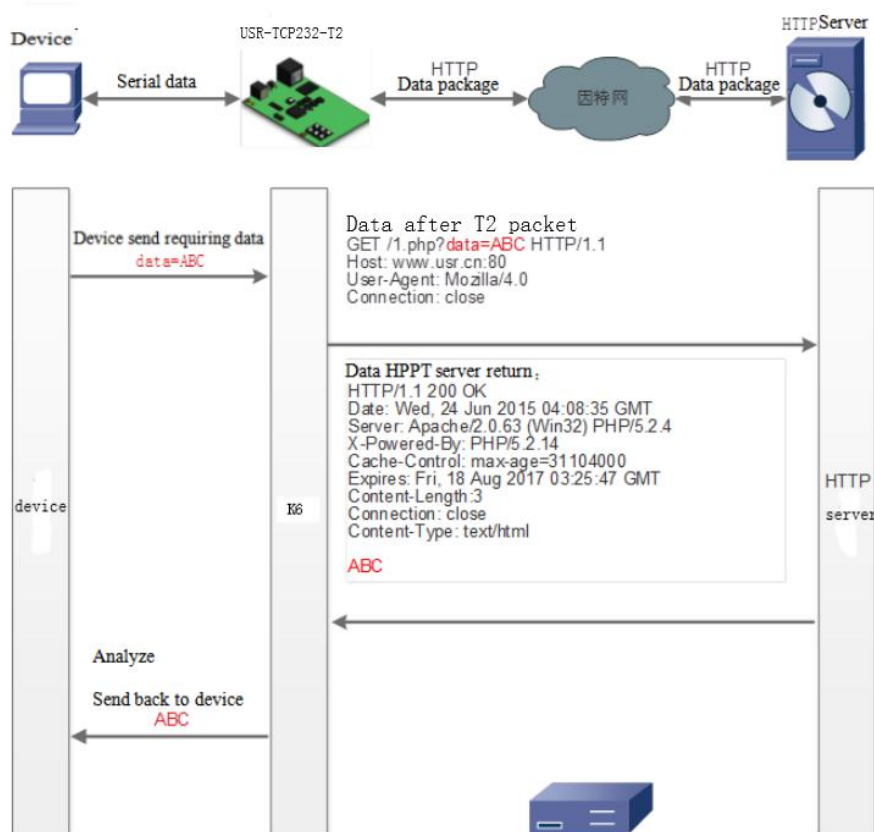
Diagram 4.2.5-1 HTTPD client
