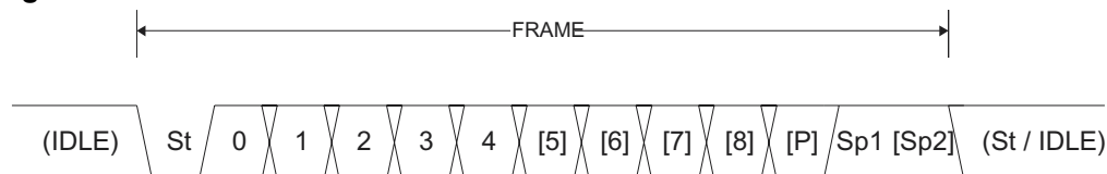
Figure 72. Frame Formats
