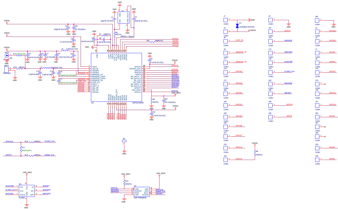
Figure 3: ESP32-WROVER Schematics
