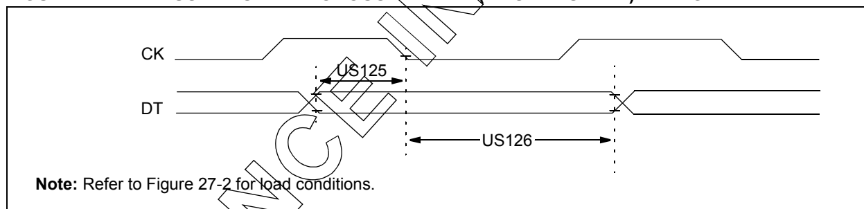
FIGURE 27-14: USART SYNCHRONOUS RECEIVE (MASTER/SLAVE) TIMING
