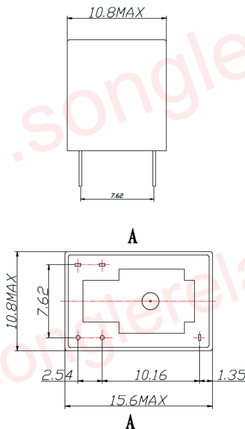
(Bottom view )
