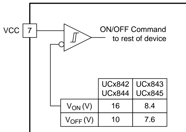
Figure 15. UVLO Threshold
